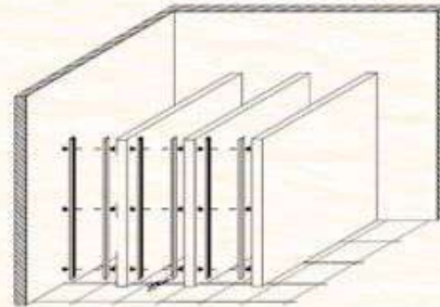
2) Install the aluminium sub-frame for the door
