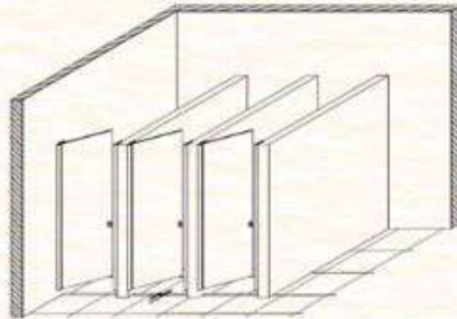
5) The last step involves installing the door panel along with all required accessories
